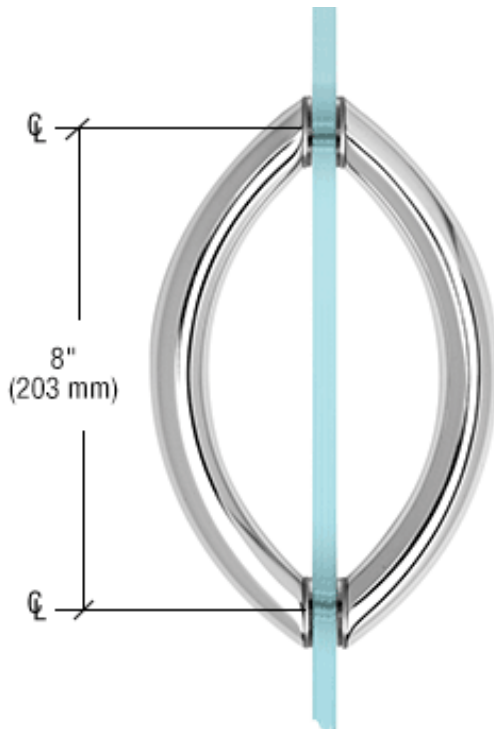
CSH8x8 8" Crescent Style Back-to-Back Pull Handles Without Metal Washers
