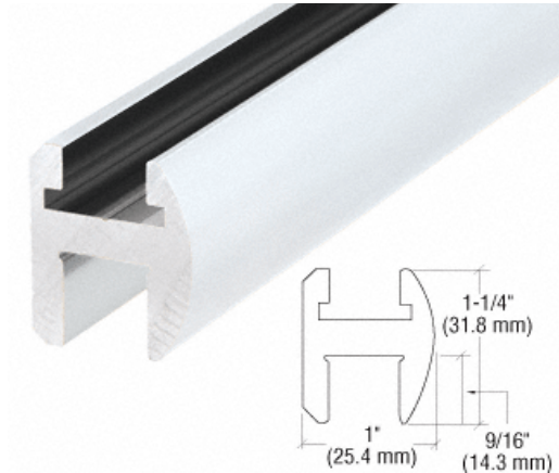
Standard Header Trim
