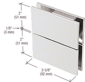
Glass to Glass Transom Hinge
