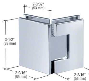
135 Glass to Glass Hinge
