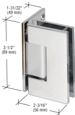
Offset Hinge
