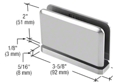
Top or Bottom Mount Hinge
