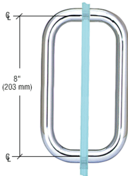
BPD8 8" Back-to-Back D-Pull 3/4" Diameter Pull Handles *Can be specified With or Without Metal Washers
