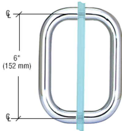
BPD6 6" Back-to-Back D-Pull 3/4" Diameter Pull Handles *Can be specified With or Without Metal Washers
