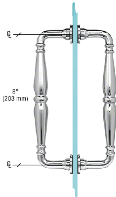
V1C8X8 8" Victorian Style Back-to-Back Pull Handle
