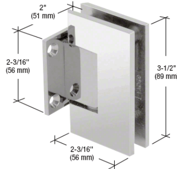
Short Back Plate Hinge
