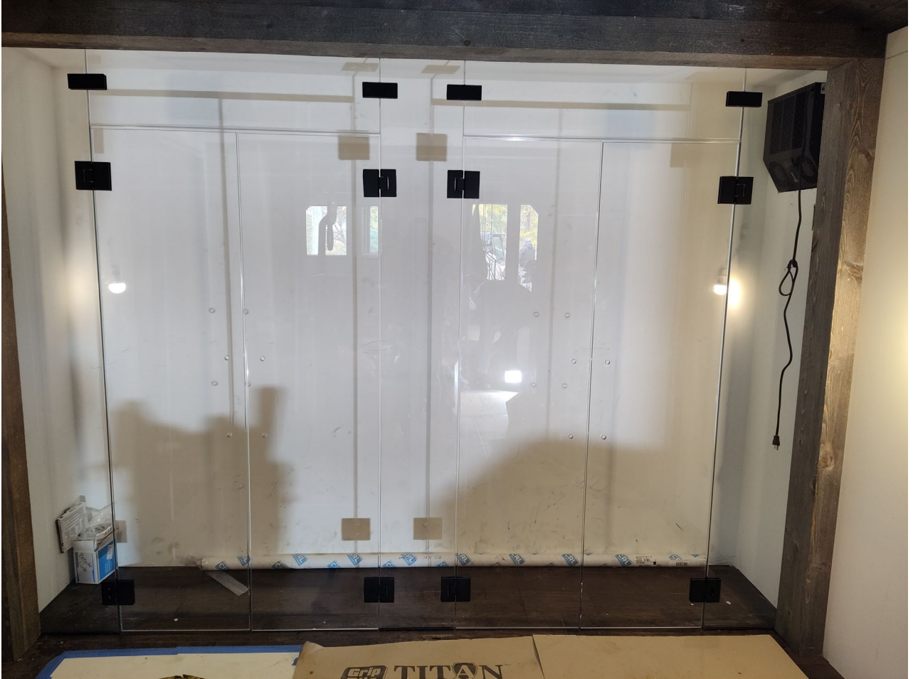
Custom Wine Room Enclosure Glass Application: Low Iron; 1/2" Tempered Glass (Required)
